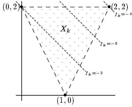
(a) X_k and contours of f_k(x, y_k^{(2)}) .
