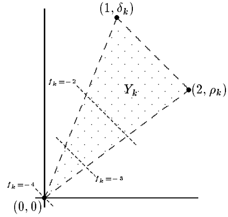
(c) Y_k and contours of f_k(x_k^{(2)}, y) , \delta_k = 5/2, \rho_k = 3/2 .
