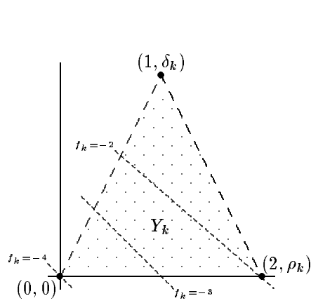
(b) Y_k and contours of f_k(x_k^{(2)}, y) , \delta_k = 2, \rho_k = 0 .
